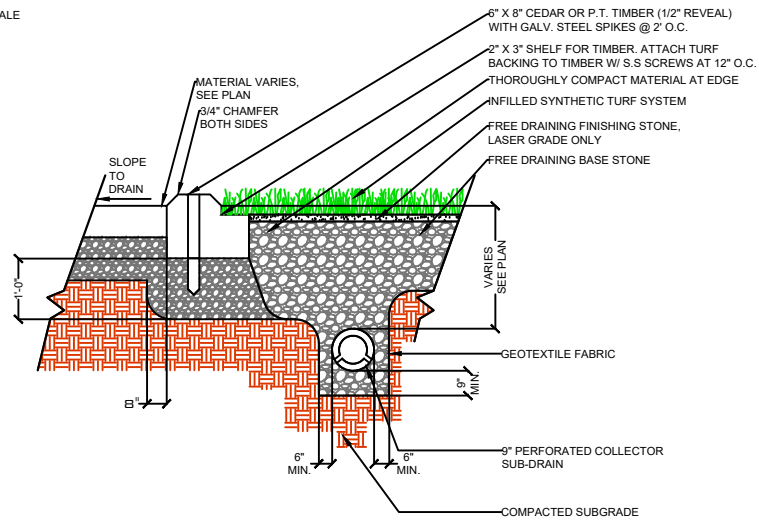
NAILER BOARD
